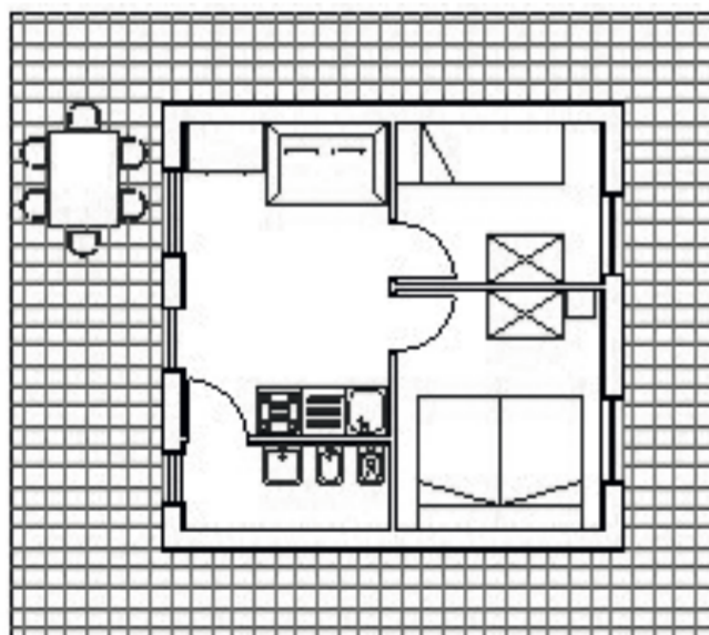
THREE-ROOMS BUNGALOWS sqm. 30 + 10 of veranda
